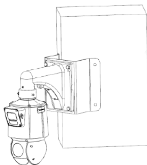
Corner Mount XLGUC08 + XLGJB12 + XLGWE45
